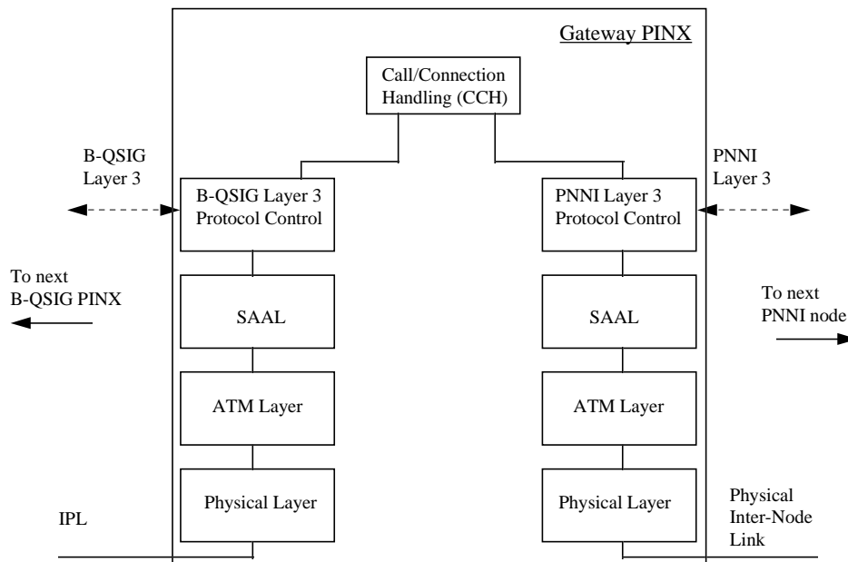
Figure L-2 - Signalling protocol model for B-QSIG/PNNI interworking
