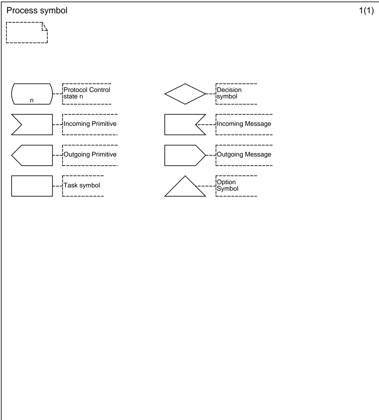
Figure D.1 - Key to symbols used in the Protocol Control SDL diagram
